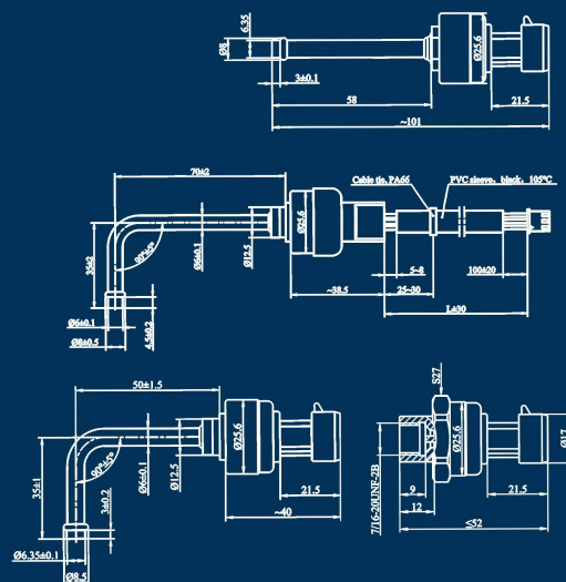
产品尺寸图 DIMENSIONAL DRAWING
